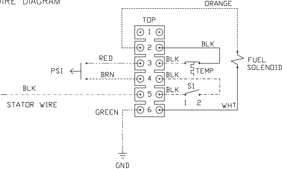
WIRE DIAGRAM
